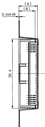
SECT. E-E
