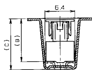
SECT. F-F
