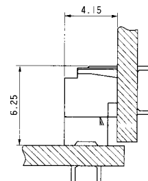
嵌合状態図 (Mating Condition)
