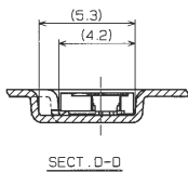
SECT. D-D
