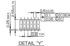
DETAIL "Y"
